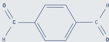
Terephthalaldehyde
