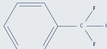
98% Yield
