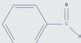
Benzaldehyde
