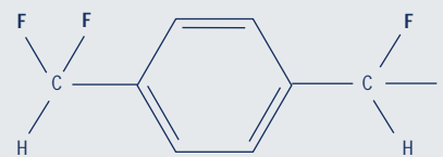
1,1,1',4',4'-Tetrafluoro-p-xylene 96% Yield
