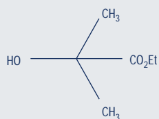
Ethyl-2-Hydroxybutyrate
