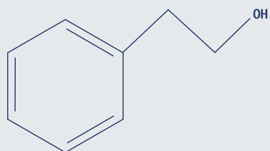
Phenethanol
